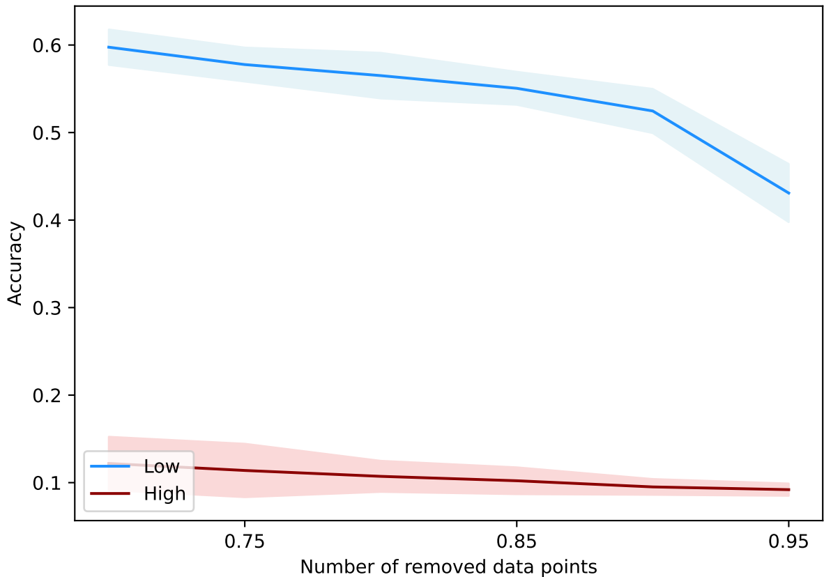
DataAttrOpt(5000, 0.03, 15, best, +b, alpha=best) - cifar10-embedding
